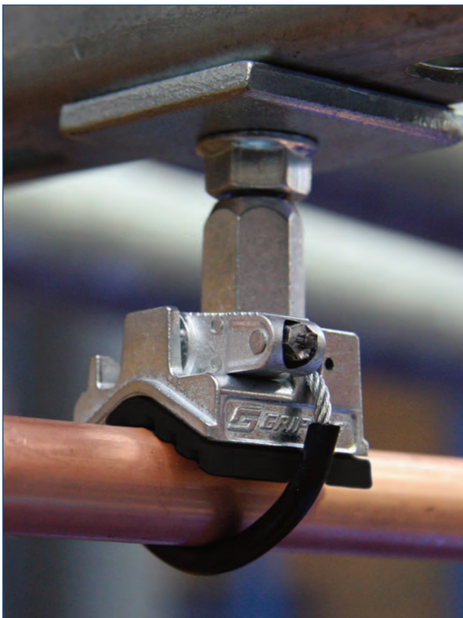
Universal Pipe Ring on Copper (With acoustic insulation)
