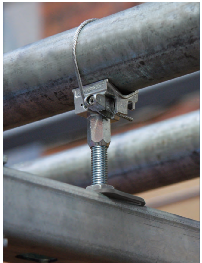
Universal Pipe Ring on Steel (Without acoustic insulation)
